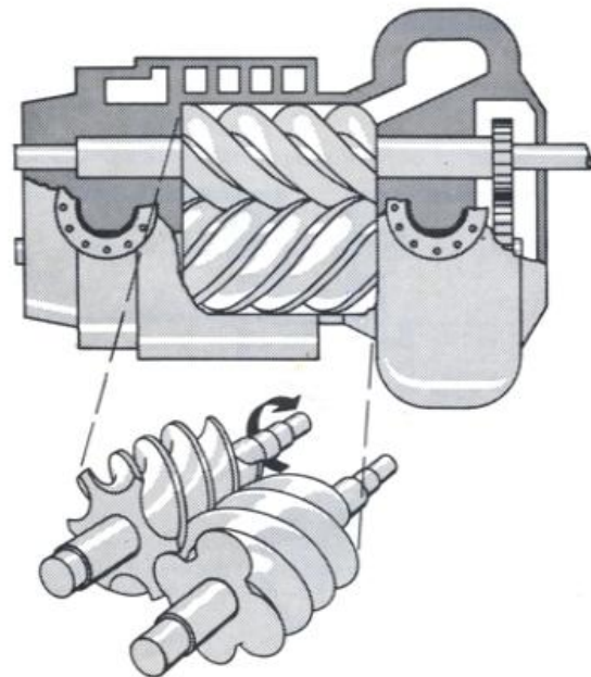
DRY SCREW COMPRESSOR
