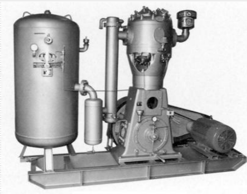
SINGLE-STAGE RECIPROCATING COMPRESSOR
