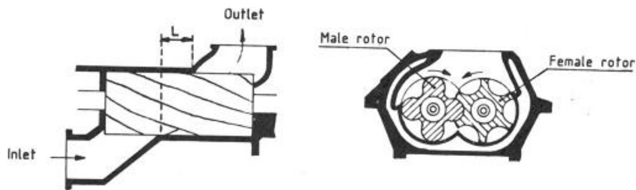
OPERATING PRINCIPLE OF THE SCREW COMPRESSOR
