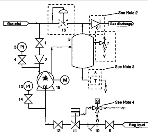
Figure A—LRVP Once Through System
