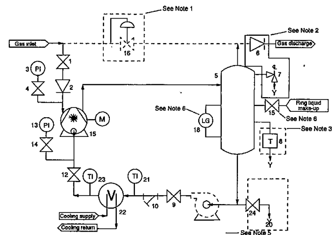
Figure C—LRVP Total Recirculation System
