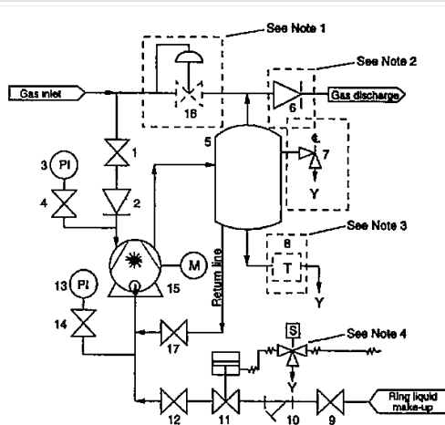
Figure B—LRVP Partial Recirculation System
