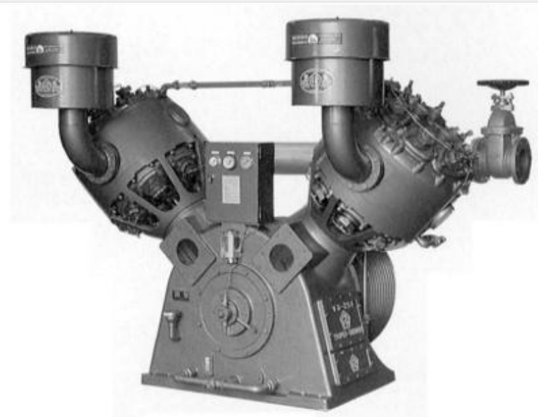
SINGLE-STAGE TWO CYLINDERS RECIPROCATING COMPRESSOR
